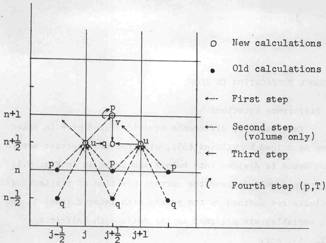
Fig.5.2.--Computational Sequence
