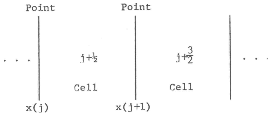
Fig. 5.1.--Difference Scheme in Space
